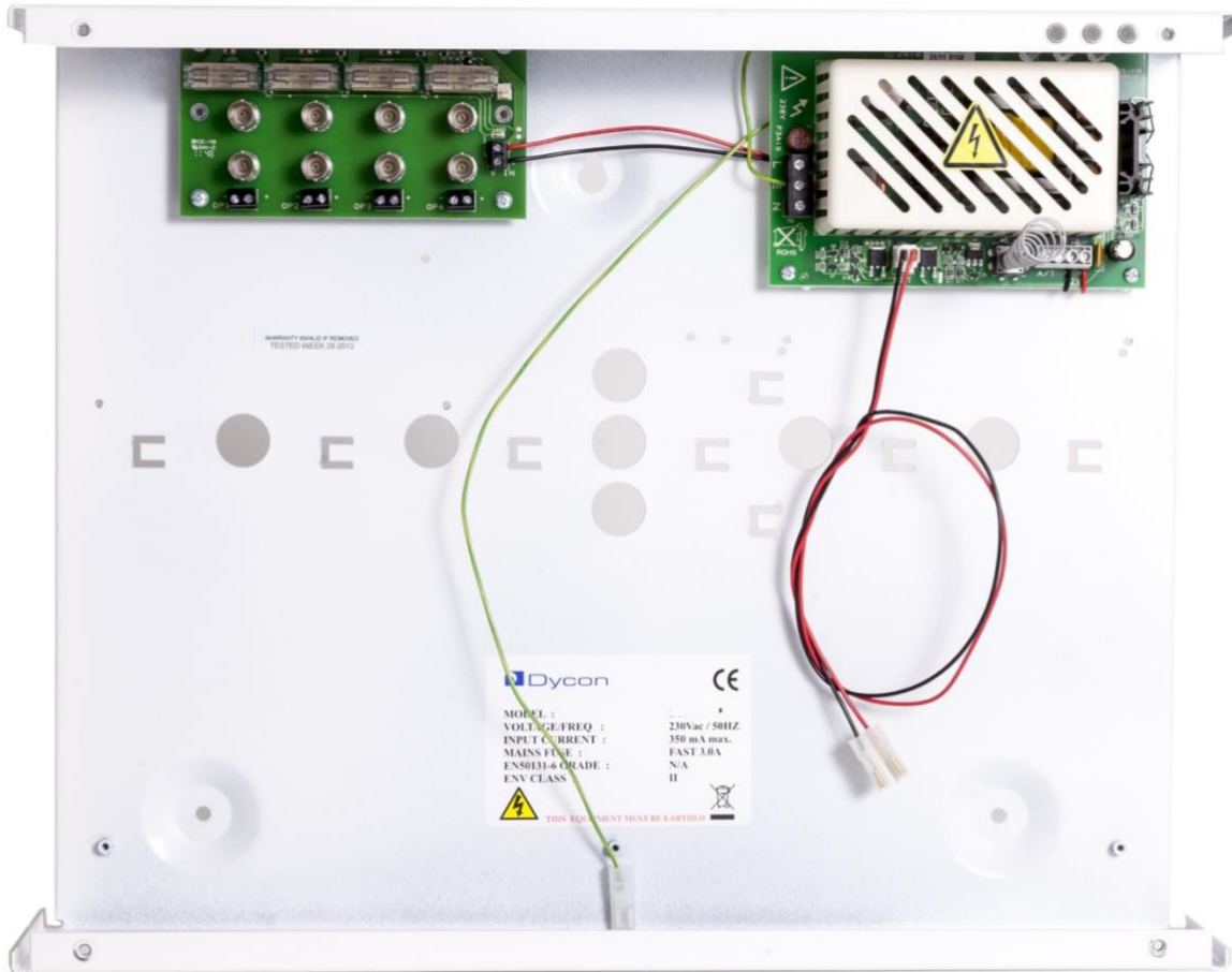
The illustration shows a D1543C fitted with an optional D15X4-BNC video output power splitter
